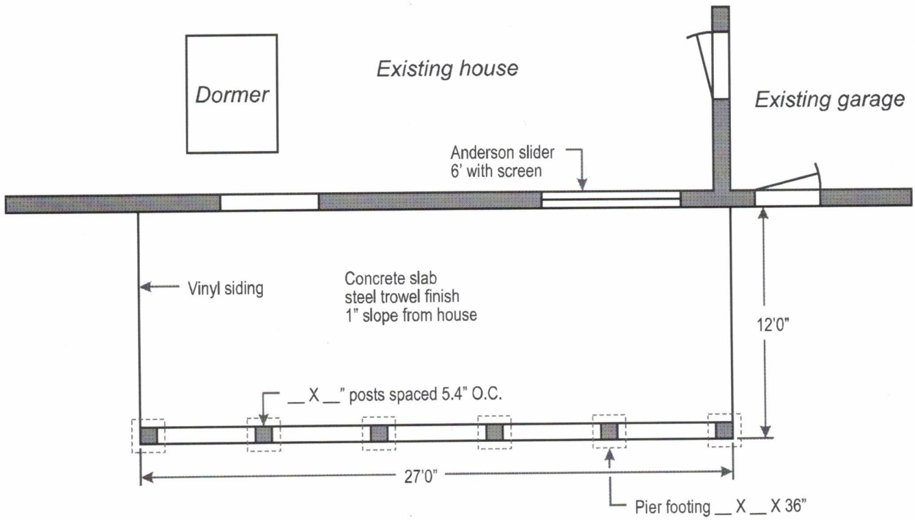
Floor Plan
